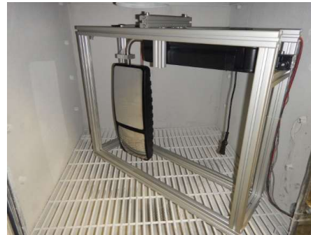
Folding actuation of an agricultural outside mirror
