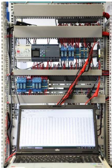
Measurement test rack
